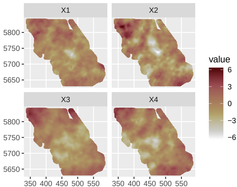
Sample from the fitted model
