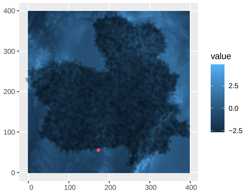
Figure 3: Integration scheme for numerical approximation of the stochastic integral in La Mancha Region
