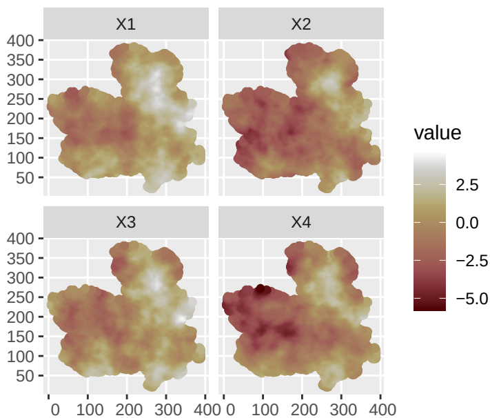
simulated spatial fields
